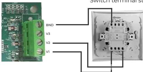
Two speed connection block on the PCB
