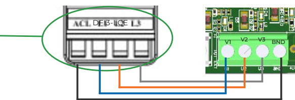
Control terminal strip
