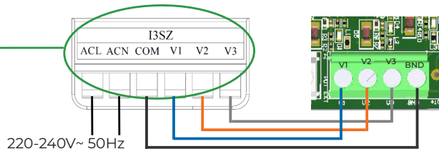
Three speed connection block on the PCB
